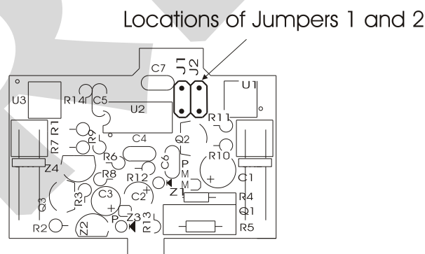
Figure 25 - Place of jumpers in analog output board
