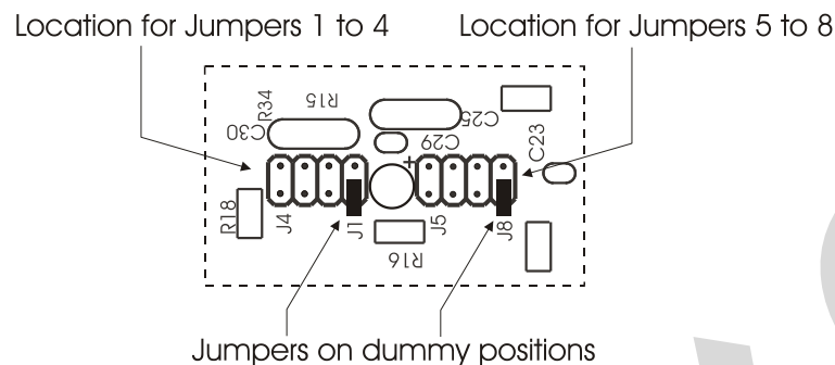
Figure 21 - Jumpers not used for 0 to 10V input placed in the board connector
