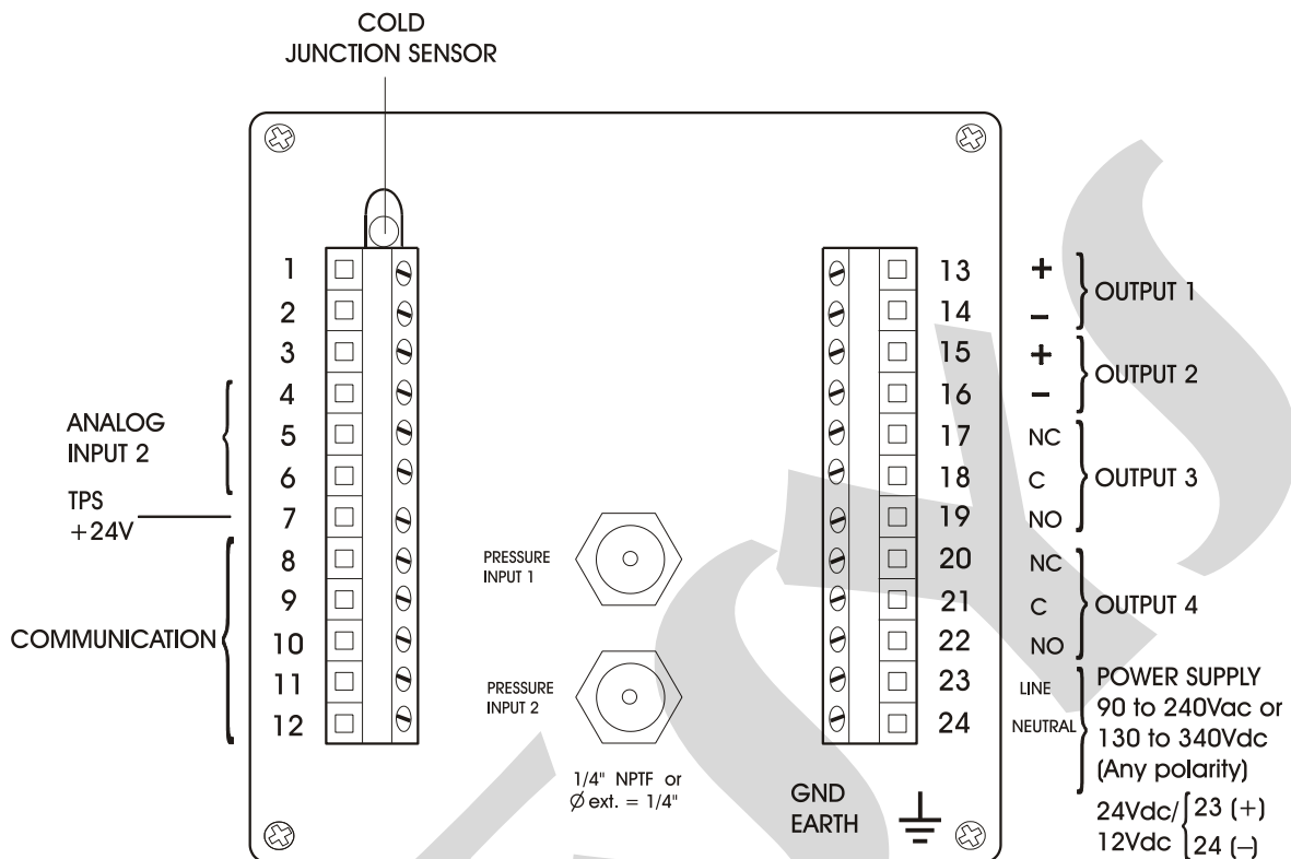
Figure 3 - Indicator Terminals
