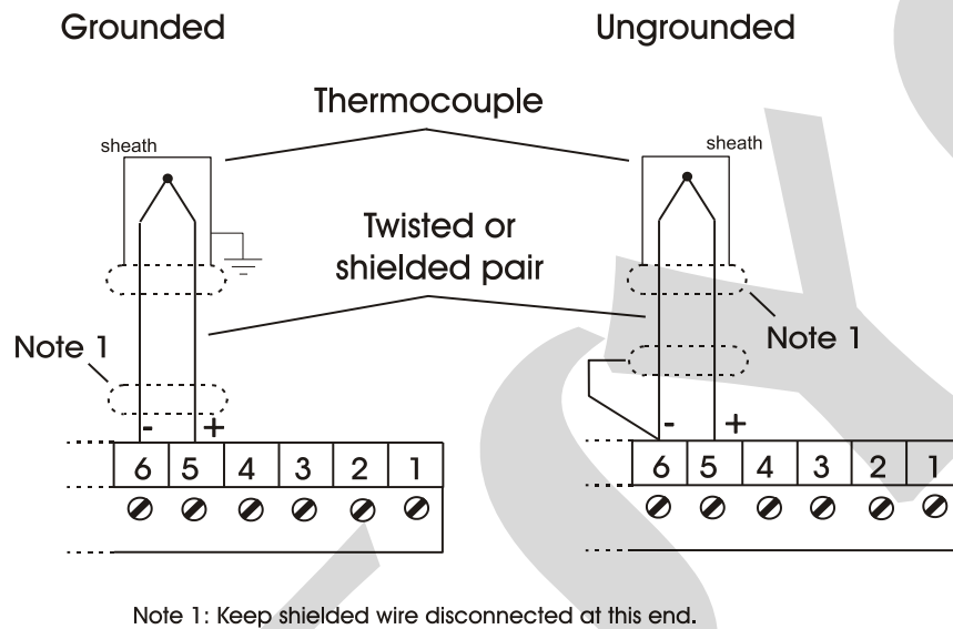
Figure 4 - Thermocouple Input
