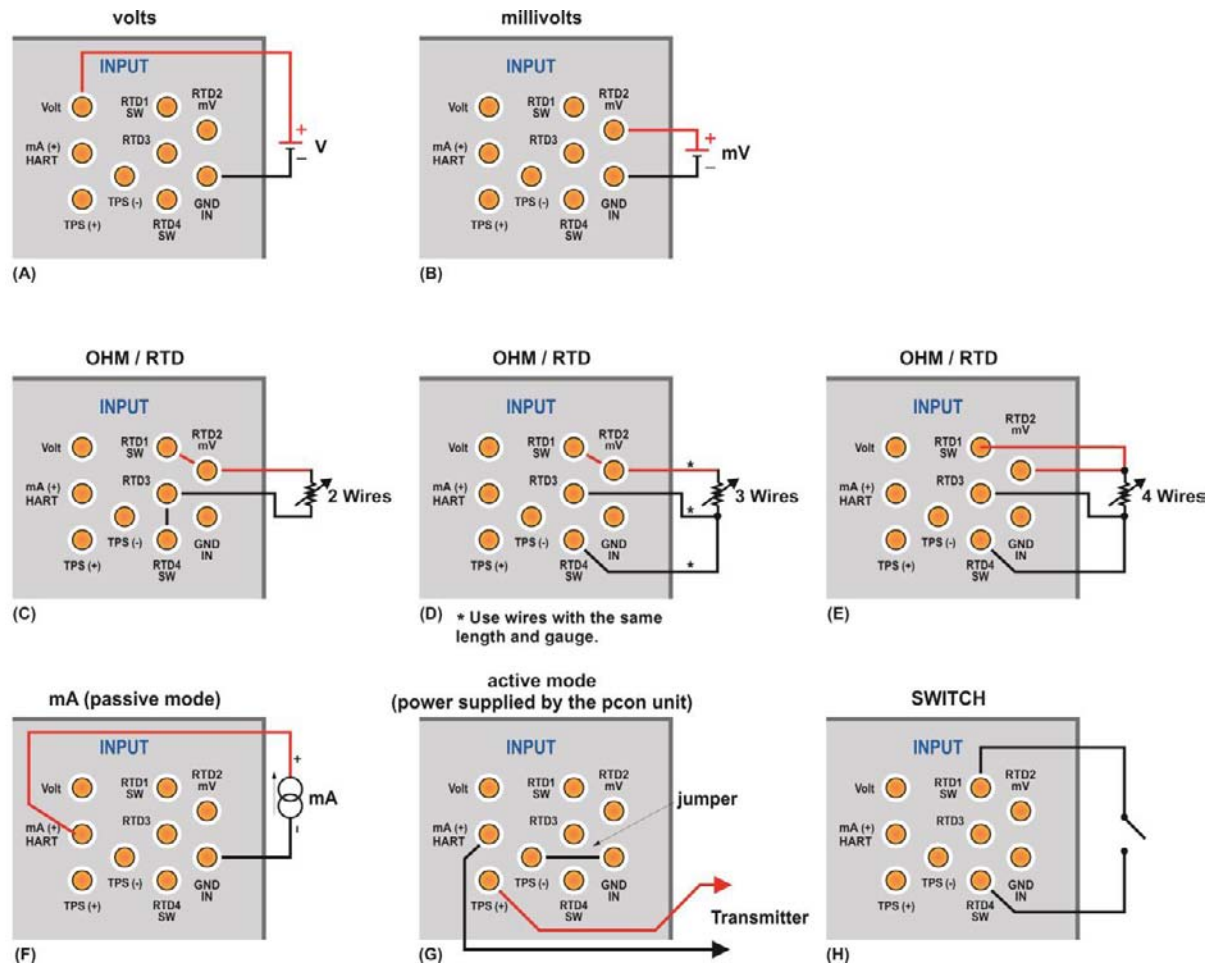
Fig. 40 – Auxiliary Input Connections.
