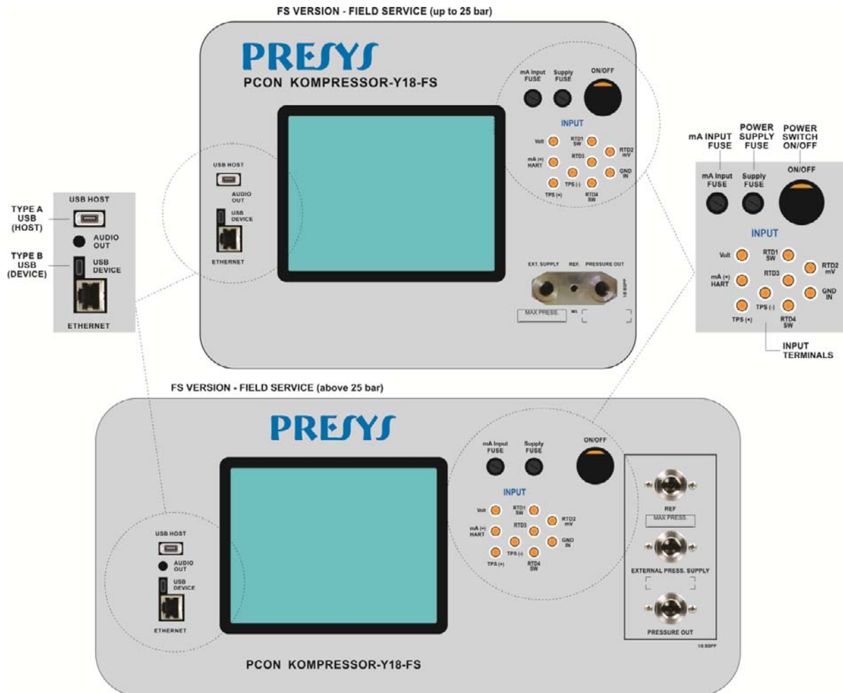
Fig. 03 – FS Version - Field Service Front Panel
