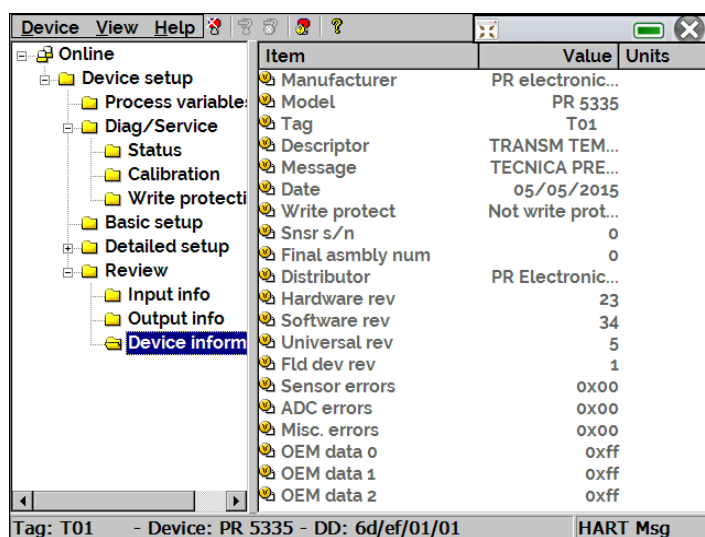
Fig. 66 – Device Parameters.
