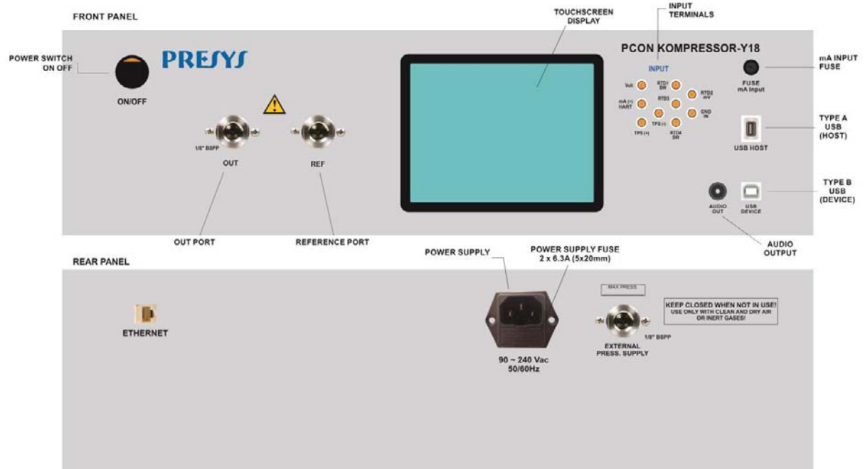
Fig. 01 – RM Version- Rack Mounting
