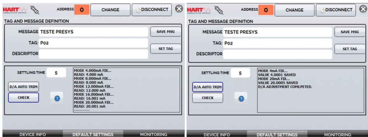
Fig. 65 – Checking / Adjusting the mA HART® Transmitter Output.
