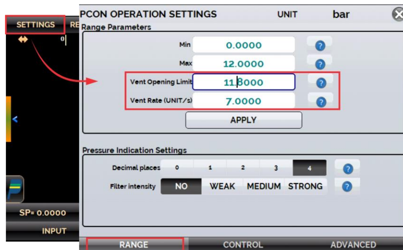
Fig. 33 – VENT Configuration
