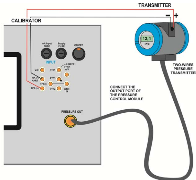
Fig. 46 – Pressure Transmitter Calibration.
