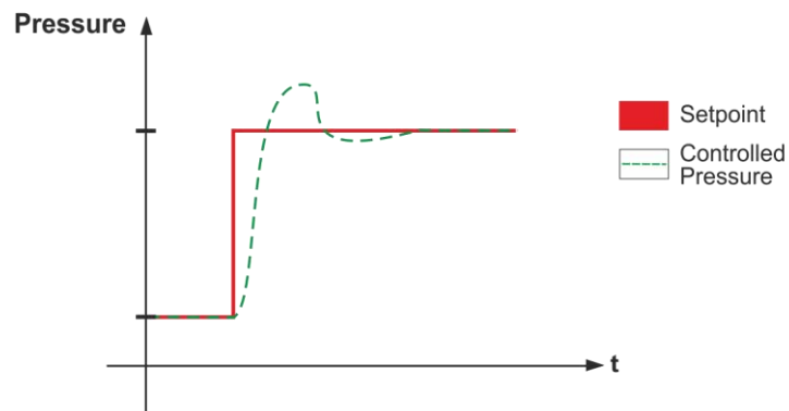
Fig. 22 – Max control mode.
