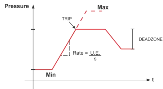
Fig. 49 – Pressure Switch Test Result
