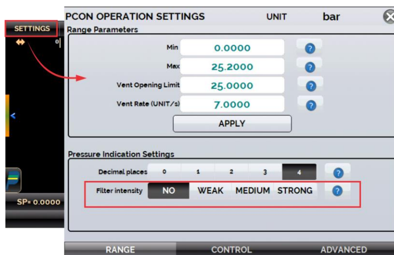
Fig. 36 – Filter Intensity.
