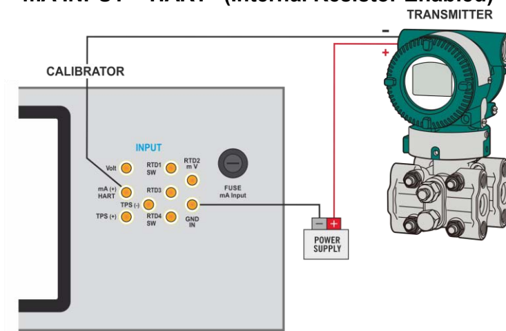
Fig. 58 – Transmitter powered up by the Calibrator (TPS) mA INPUT + HART® (Internal Resistor Enabled)
