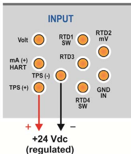
Fig. 41 – TPS Power Supply.
