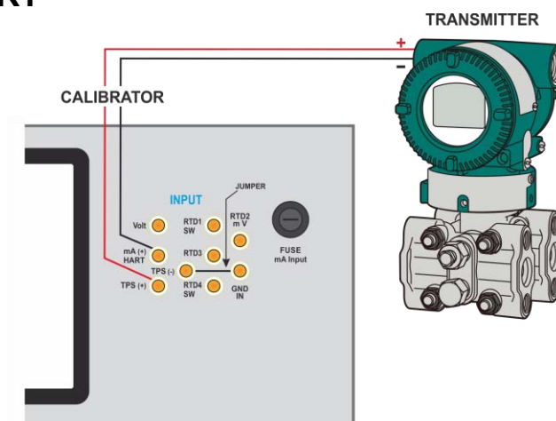
Fig. 58 – Transmitter powered up by the Calibrator (TPS) mA INPUT + HART® (Internal Resistor Enabled)
