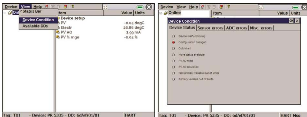
Fig. 68 – Device Status.
