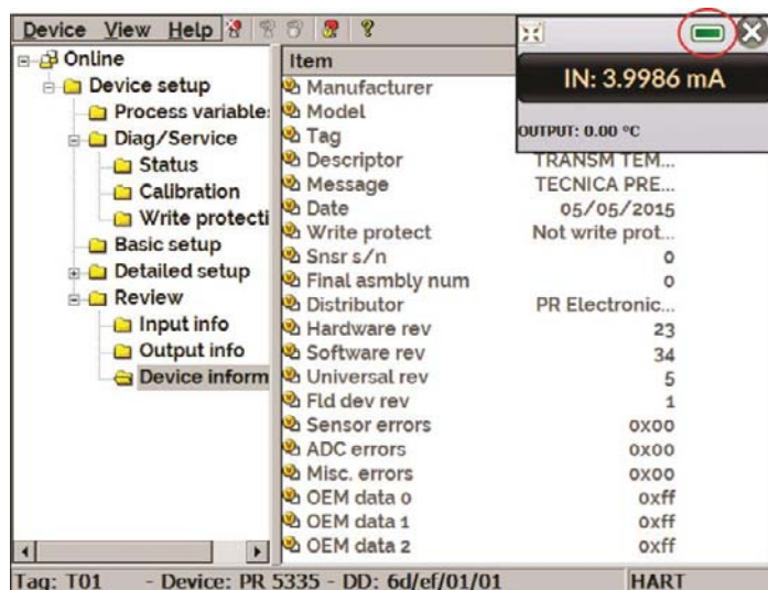
Fig. 67 – Calibrator / Controller Input and Output Values.
