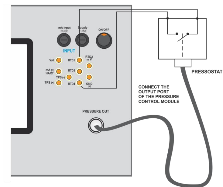
Fig. 47 – Pressure Switch Verification.
