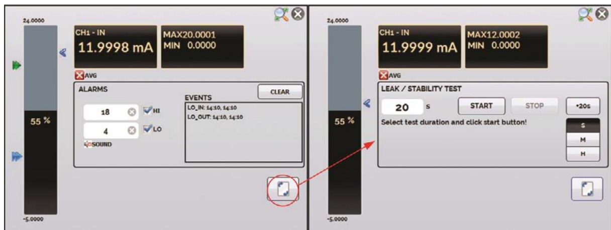
Fig. 52 – Leak/stability test screen.
