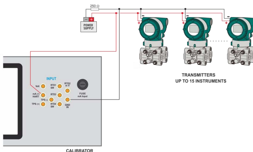
Fig. 60 – ONLY HART®
