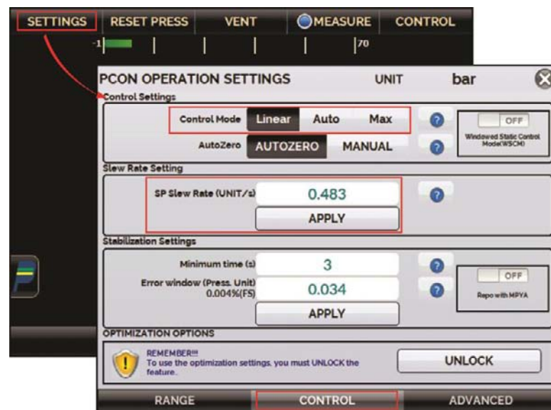
Fig. 23 – Control Settings - External Pressure Supply Mode
