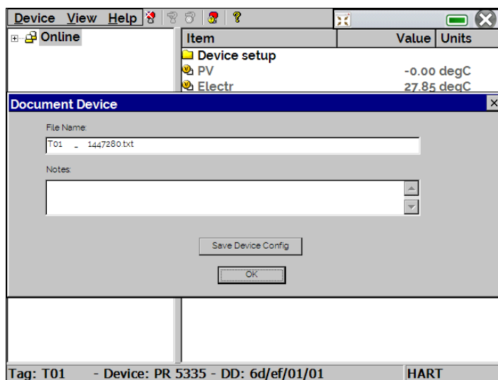
Fig. 69 – Saving the Configuration of a Device
