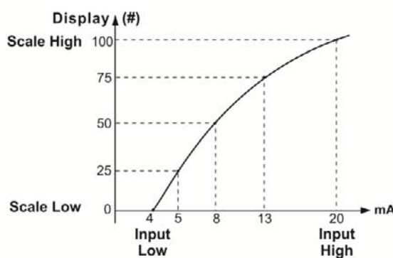
Fig. 45 – SCALE Function (FLOW)
