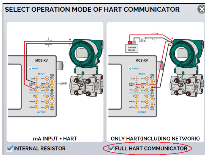
Fig. 61 – ONLY HART®
