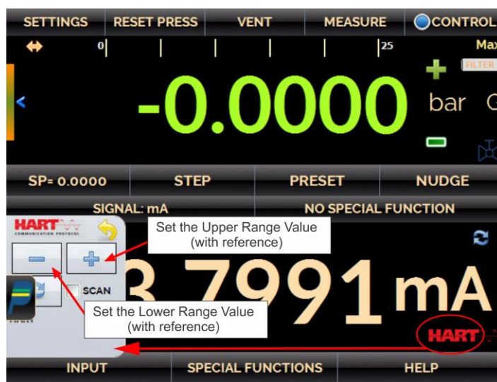
Fig. 63 – Quick HART® Adjustment with Reference.
