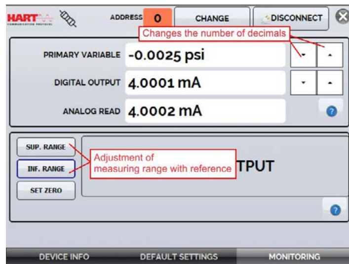
Fig. 64 – Adjusting the Measurement Range of the HART® Transmitter with Reference.
