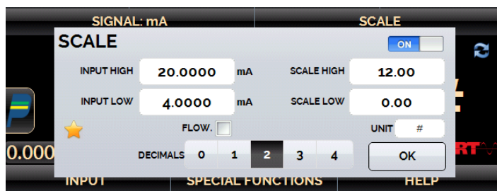
Fig. 43 – SCALE Function (LINEAR)
