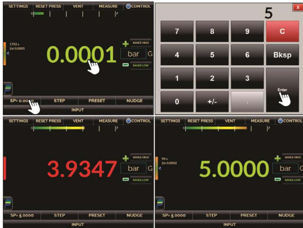
Fig. 18 – Changing the setpoint value in the CONTROL mode.
