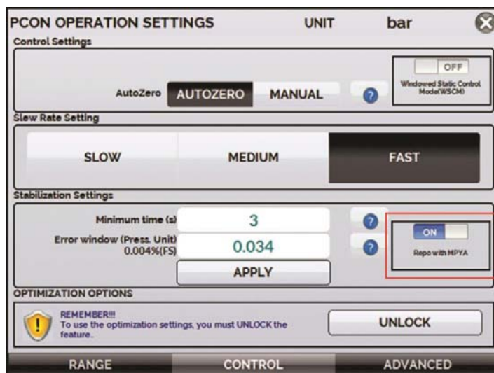
Fig. 57 – Control Mode with MPYA
