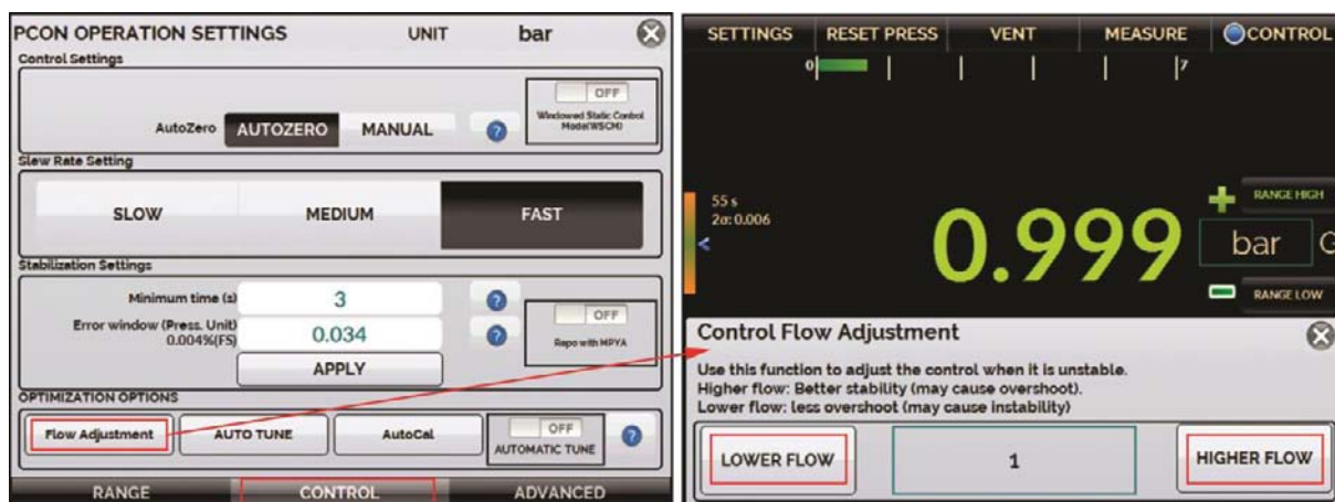
Fig. 25 – Control Optimization Options
