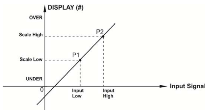
Fig. 44 – SCALE Function (LINEAR)
