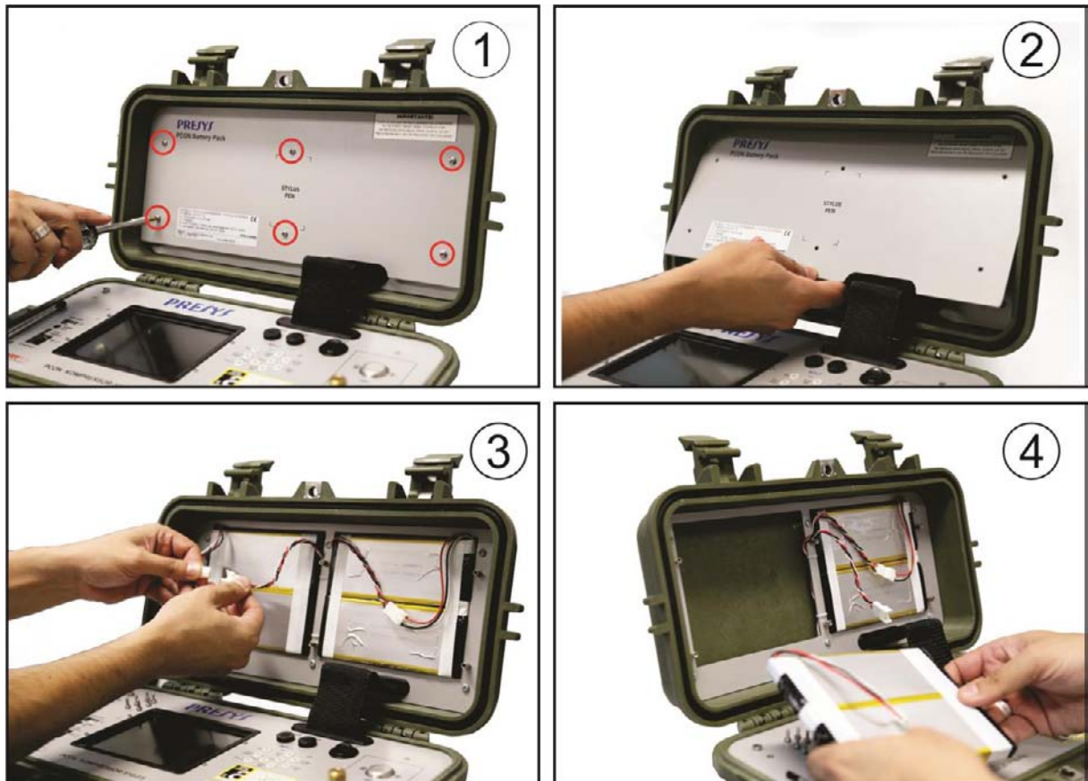
Fig. 82 – Replacing Battery Pack - FS Version over 25 bar
