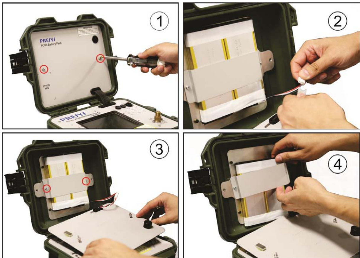
Fig. 81 – Replacing Battery Pack - FS Version up to 25 bar
