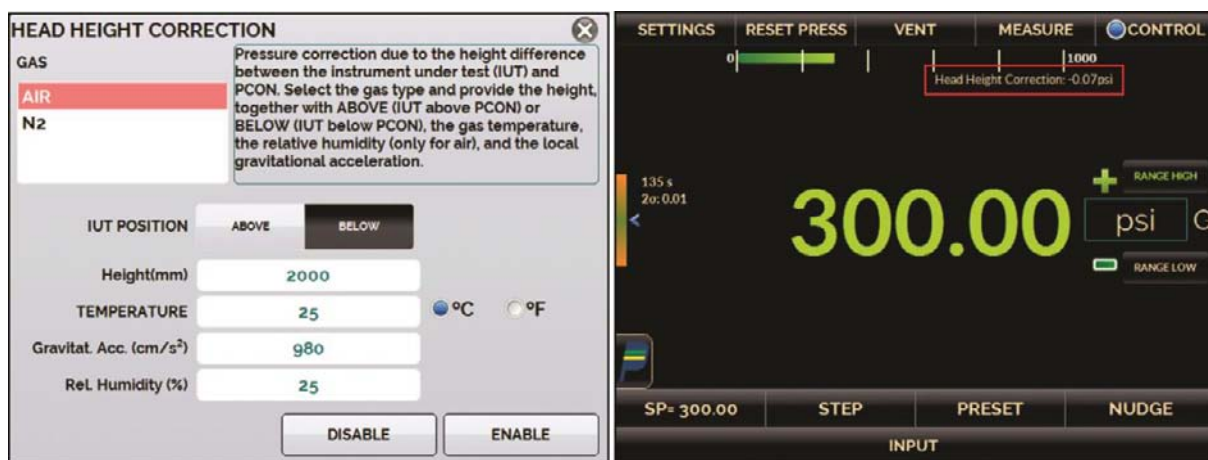
Fig. 13 – Head Height Corretion
