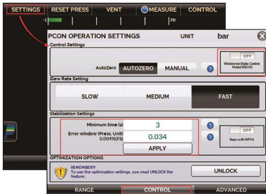
Fig. 19 – Stabilization Settings.
