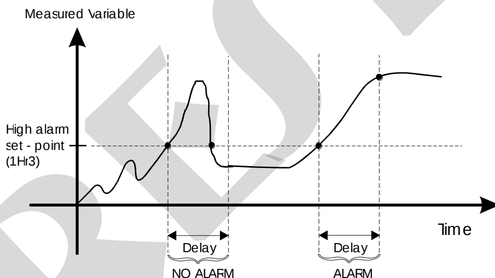
Fig.18 - Relay with delay
