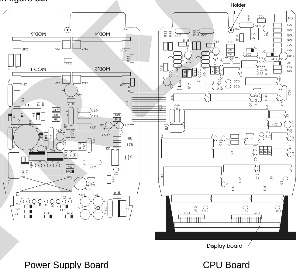
Fig. 32 - Controllers Hardware
