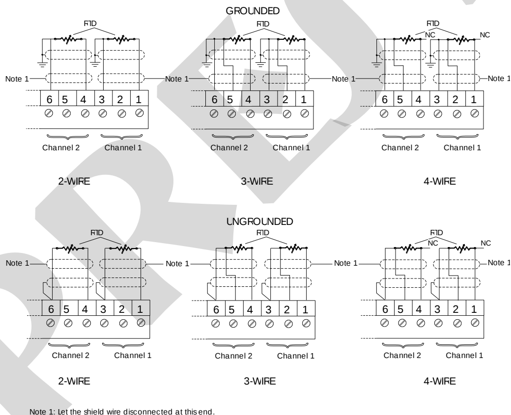
Fig. 5 - RTD Connection
