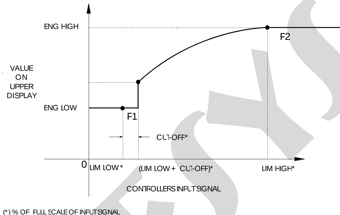
Fig. 16 - Square root of input signal
